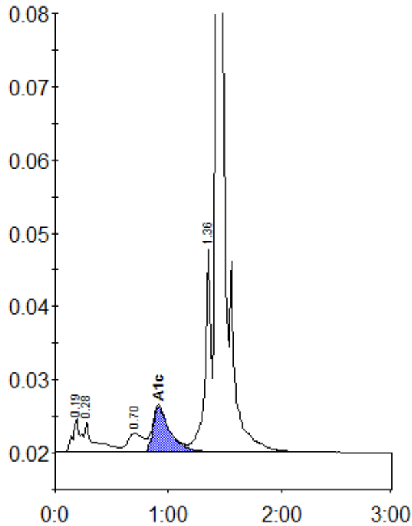
Peak table - ID: 10470063
